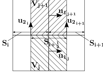
Figure 2: Staggered grid: Surfaces and velocities.
